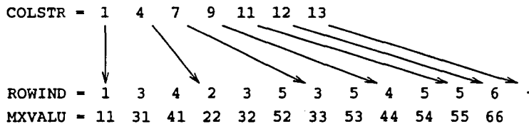
Figure 8-4: Column Pointer, Row Index Sparse Matrix Representation
