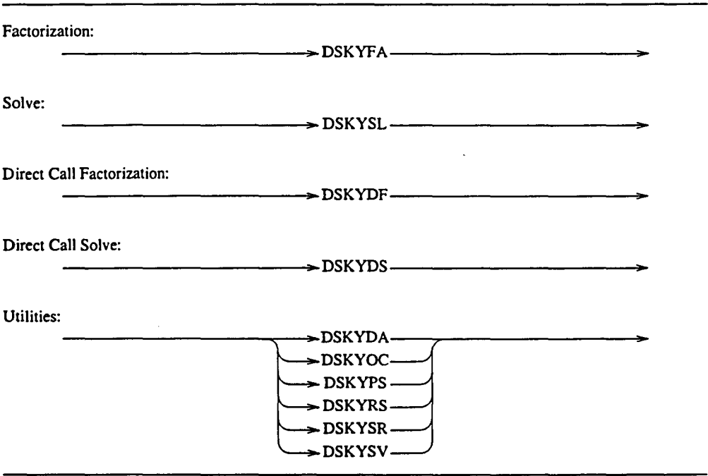
Figure 8-5: Paths of Control (Continued)
