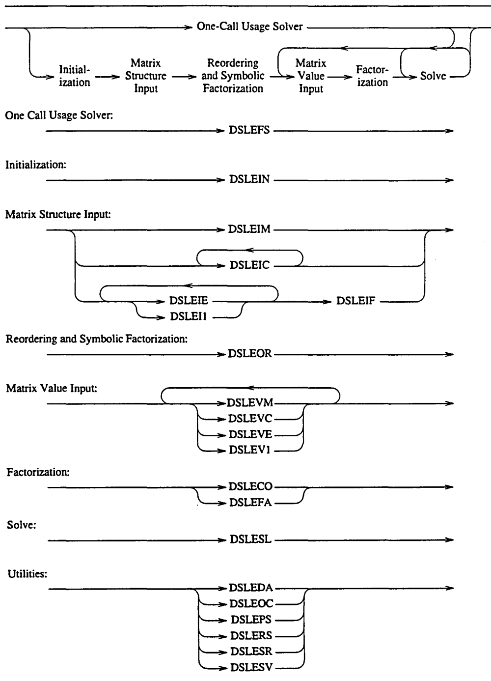
Figure 6-3: Paths of Control
