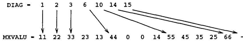
Figure 8-3: Reverse Skyline Matrix Representation
