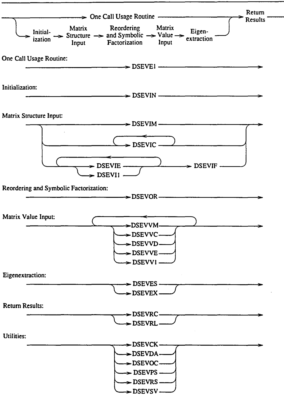
Figure 7-3: Paths of Control
