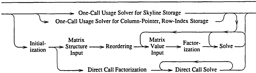
Figure 8-5: Paths of Control
