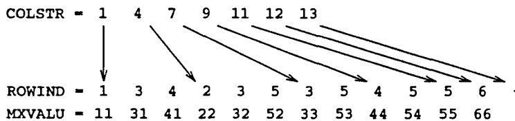
Figure 7-2: Column Pointer, Row Index Sparse Matrix Representation
