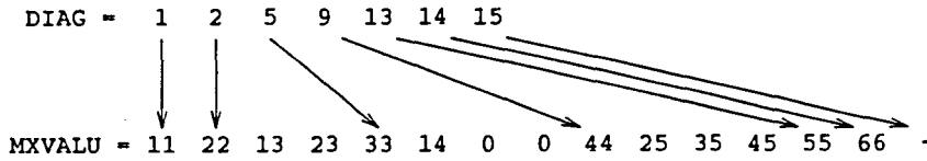
Figure 8-2: Skyline Matrix Representation
